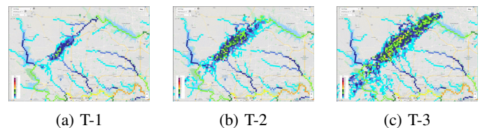
Fig. 2: RDHM generated streamflow
