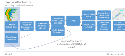
Fig. 1: RDHM Workflow Diagram
